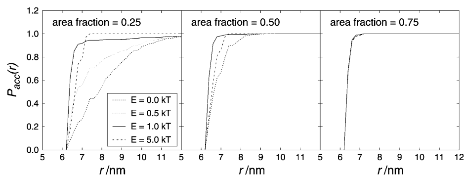
FIGURE 8 Similar to Fig. 7, but here the NNDA is shown for interacting particles with different interaction energies, E , and different particle densities. For clarity, error bars are not shown.
