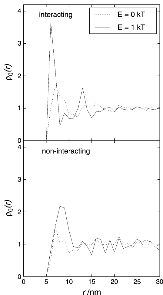
FIGURE 15 Influence of noninteracting spheres on the arrangement of particles in the membrane. The area occupation is 0.50 and 20% of the particles are noninteracting. The PCA for E = 0 kT and the arrangement resulting from 1 kT interaction energy is shown. (Top) Interacting spheres (LHC II). (Bottom) Noninteracting spheres ( cyt bf ).
