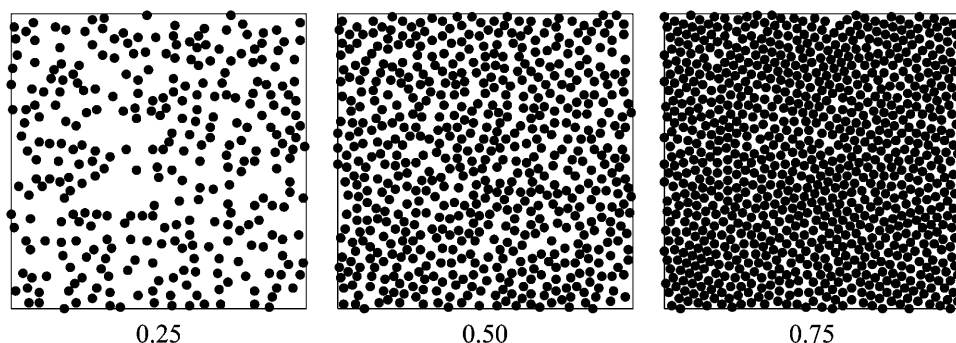
FIGURE 5 Random distribution ( E = 0 kT) of homogeneous spheres on a square lattice. The occupied area fraction is 0.25, 0.50, or 0.75. The diameter of the spheres is 6.25 nm and the lattice size is 200 \times 200 nm.
