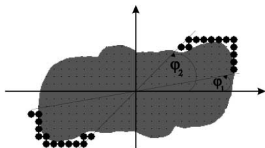
FIGURE 3 Binding sites on PS II. Binding sites are shown as solid circles. The angles \phi_1 and \phi_2 (here 10^\circ and 45^\circ ) determine the position of the binding sites.
